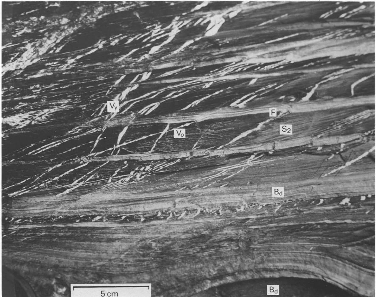
Fig. 2. Photograph of the outcrop studied, looking south. B_d —bedding with refracted veins; F —folded bedding associated with veins in the closure; V_o and V_y —calcite veins; S_2 —main foliation.
